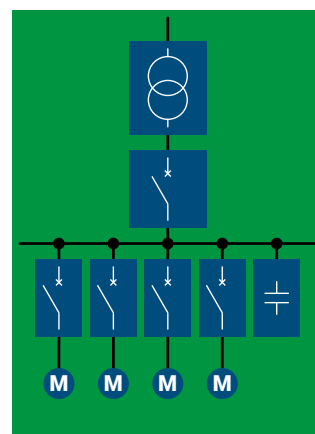
Central compensation
