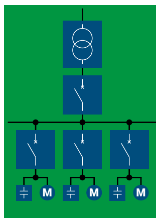
Individual compensation
