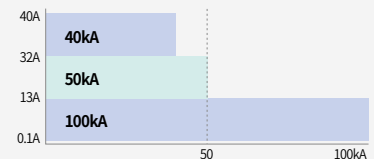
MMS-32H MMS-32HI • High break • Magnetic release
