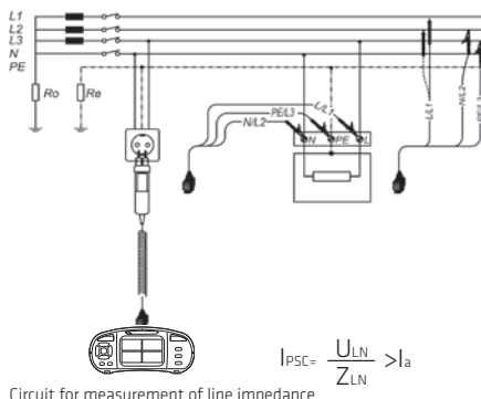
Circuit for measurement of line impedance
